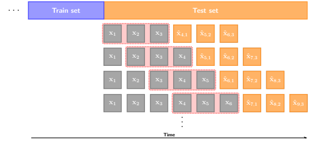
Figure 2: Illustration of the multi-horizon evaluation procedure. For each forecast origin, the red dotted rectangle denotes the measurements used for feature calculation, while the orange squares denote the resulting forecasts
