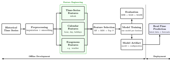
Figure 1: High-level overview of the proposed forecasting framework, showing different steps and components
