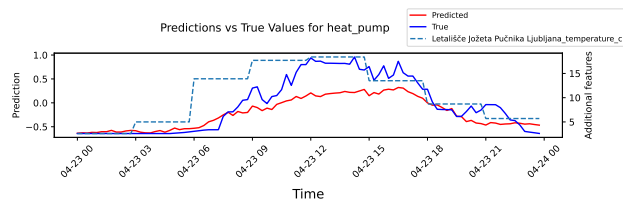
Figure 3: Example of heat pump forecasting for one day. The red line represents the predicted and the blue line true heat pump consumption; the dashed line is the temperature forecast used as an exogenous input
