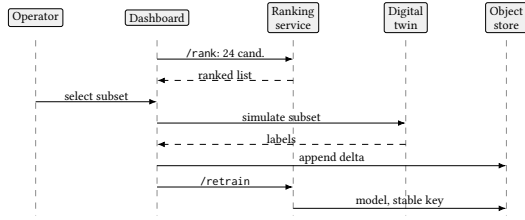
Figure 1: Deployed human-in-the-loop active learning workflow. The operator decides which candidates are simulated; labels come from the digital twin. The ranking service ranks from its own local copy of the current model, so no model is fetched from the store during a call.
