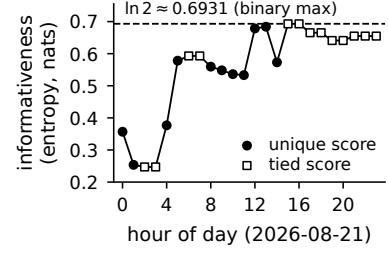
Figure 2: Informativeness scores returned by /rank for the twenty-four candidate hours of 2026-08-21, in clock order rather than rank order. Open markers denote tied candidates; the dashed line is the maximum \ln 2 for a binary classifier.
