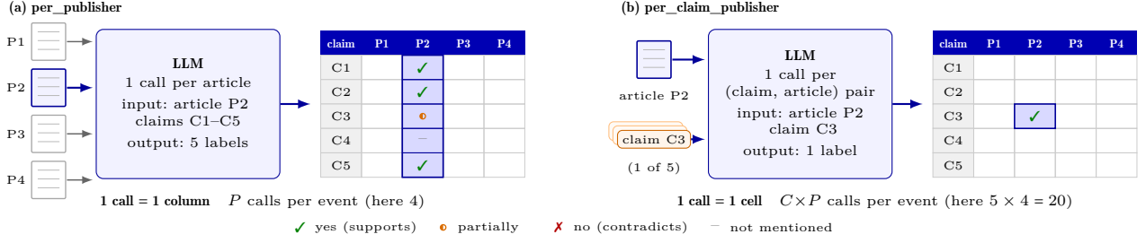
Figure 1: Illustrative classification architectures on a hypothetical event with 4 articles and 5 claims: (a) per_publisher, one call per article for all claims; (b) per_claim_publisher, one call per (claim, article) pair.
