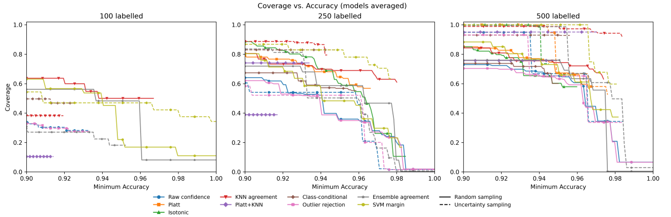
Figure 1: Coverage versus minimum accuracy for the nine criteria, one panel per checkpoint. Each curve averages the three base classifiers; solid lines show random sampling and dashed lines uncertainty sampling. At accuracy level x , the curve height is the highest coverage achievable subject to an accuracy of at least x ; criteria whose accuracy never reaches x are absent from the panel.
