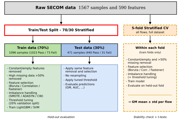
Figure 1: Preprocessing and experimental pipeline overview.
