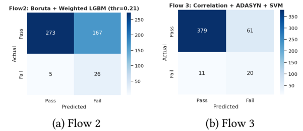
Figure 2: Confusion matrix for two of the flows to visualise the different outputs for high number of detected defects with Flow 2 and the highest GM value with Flow 3. Note that the highest recall is from Flow 6, in that case 27 defects were detected but the false positives increase with 20 compared to Flow 2, even though we only detected 1 more.
