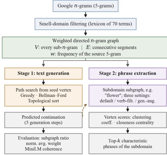
Figure 1: Overview of the methodology.
