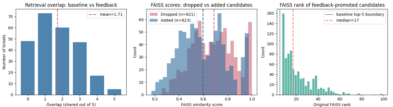
Figure 2: Feedback replaces retrieval, not reorders it. Promoted candidates have lower FAISS scores and come from deep in the FAISS ranking (median rank 17).
