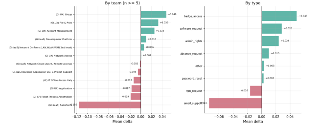
Figure 4: Mean feedback delta by team (left, teams with \geq 5 tickets) and by ticket type (right). Teal: feedback benefits; red: feedback harms.
