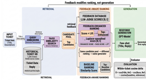
Figure 1: System architecture. Baseline and feedback differ only in the ranking of the same candidate pool.
