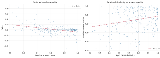
Figure 3: Left: delta vs. baseline answer quality — a clear negative trend ( r = -0.41 ): feedback helps weak baselines and hurts strong ones. Right: retrieval similarity predicts answer quality only weakly ( r = 0.24 , 6 % variance), explaining why cosine-based gating fails.
