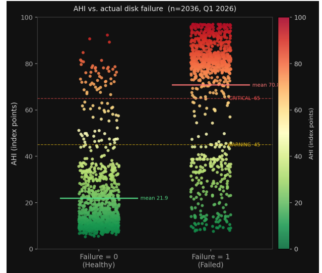
Figure 1: AHI scores for the strict-unseen evaluation from the first quarter of 2026. Each point is one daily SMART record; the vertical axis shows AHI index points.
